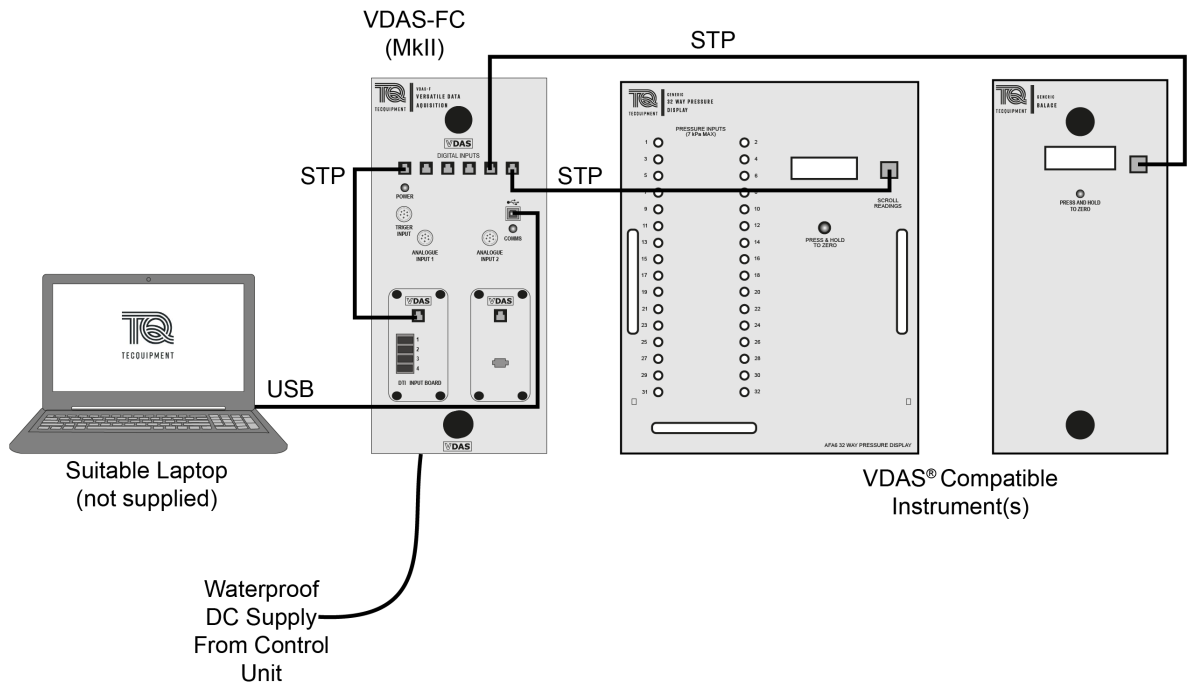
Figure 11 Typical System Connections for the VDAS-FC
