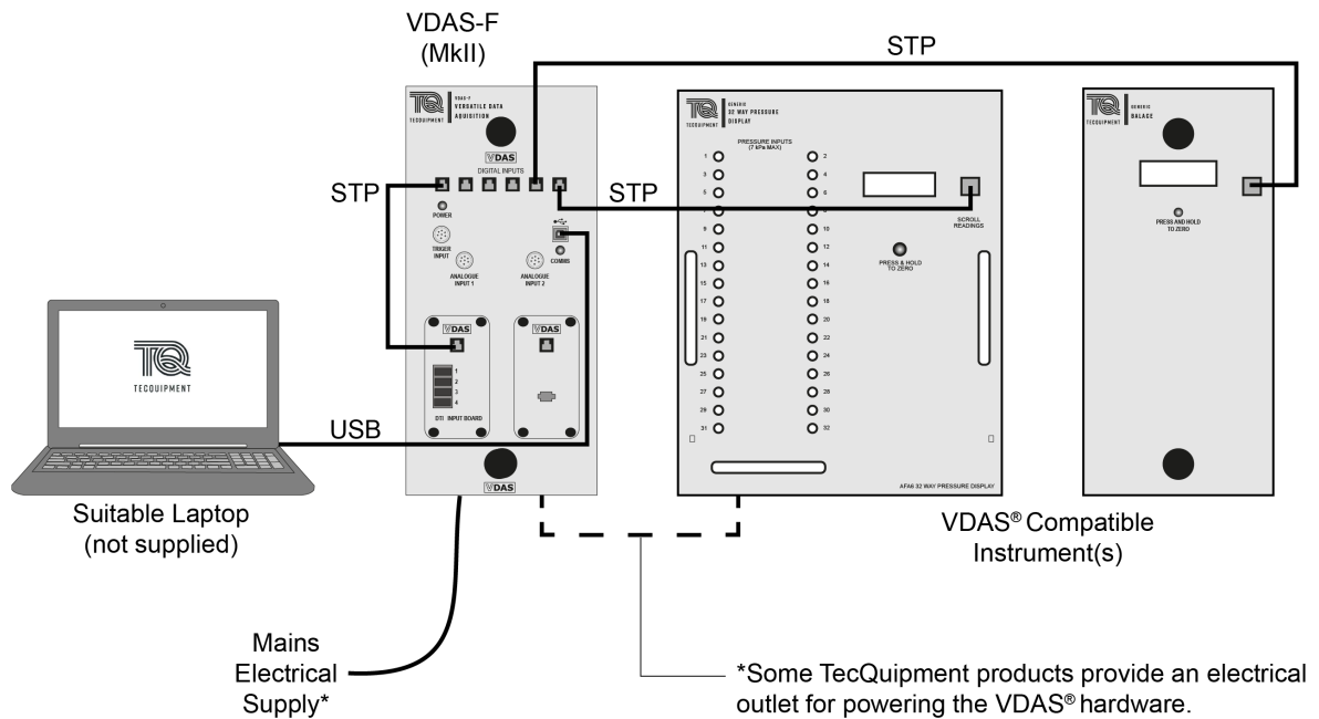
Figure 10 Typical System Connections for the VDAS-F
