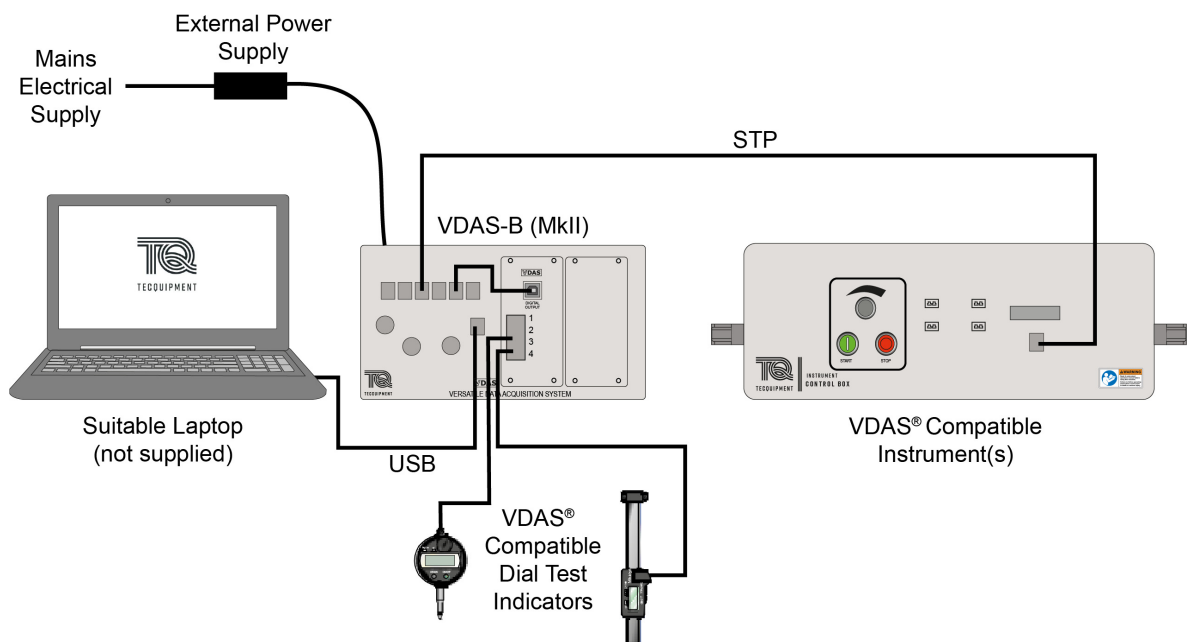
Figure 9 Typical System Connections for the VDAS-B
